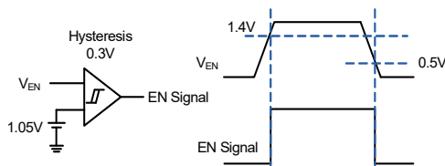
Figure 7. Enable Threshold Schematic and Timing Sequence
