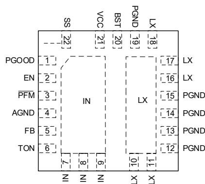
AOZ2260BQI-15 22-pin 4mm x 4mm QFN
