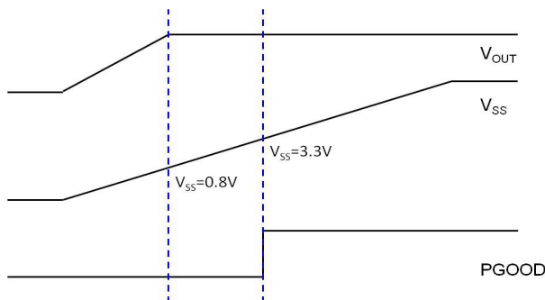
Figure 1. Soft Start Sequence of AOZ2261BQI-15
