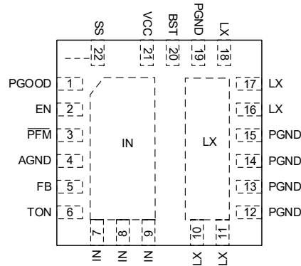
AOZ2261BQI-15 22-pin 4mm x 4mm QFN
