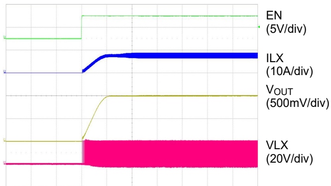
Full Load Start-up
