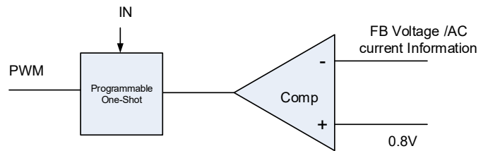
Figure 2. Simplified Control Schematic of AOZ2261BQI-18
