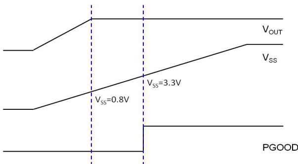
Figure 1. Soft Start Sequence of AOZ2261BQI-18
