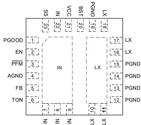
AOZ2261BQI-18 23-Pin 4mm x 4mm QFN
