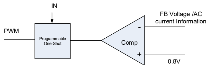
Figure 2. Simplified Control Schematic of AOZ2262BQI-15
