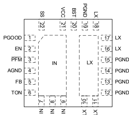
AOZ2262BQI-15 22-pin 4mm x 4mm QFN
