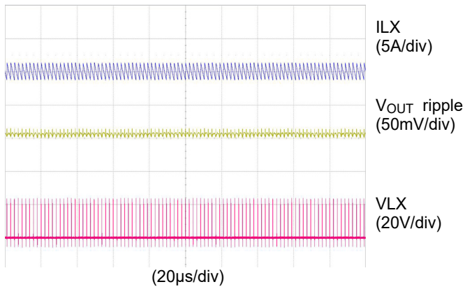
Normal Operation
