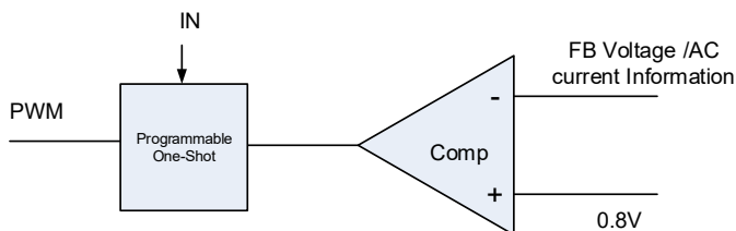
Figure 2. Simplified Control Schematic of AOZ2262BQI-28
