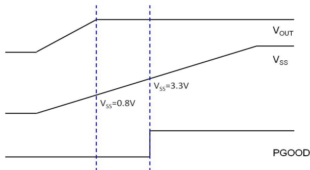
Figure 1. Soft Start Sequence of AOZ2262BQI-28
