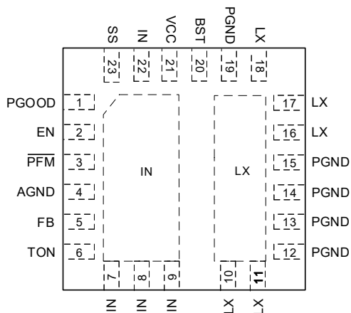
AOZ2262BQI-28 23-Pin 4mm x 4mm QFN
