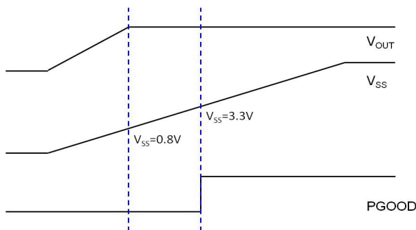
Figure 1. Soft-Start Sequence of AOZ2263BQI-15
