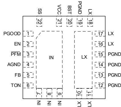
AOZ2263BQI-15 22-pin 4mm x 4mm QFN
