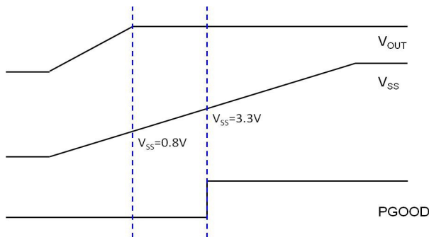
Figure 1. Soft Start Sequence of AOZ2263BQI-28
