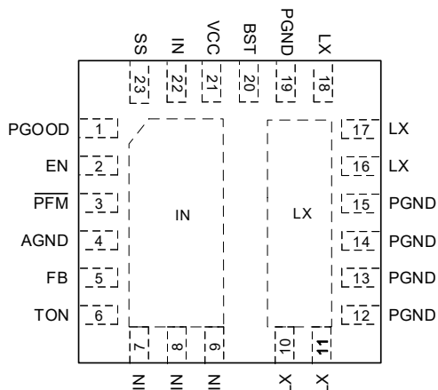
AOZ2263BQI-28 23-Pin 4mm x 4mm QFN
