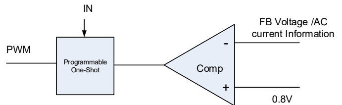
Figure 2. Simplified Control Schematic of AOZ2263BQI-28
