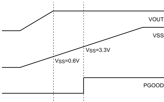
Figure 1. Soft-Start Sequence
