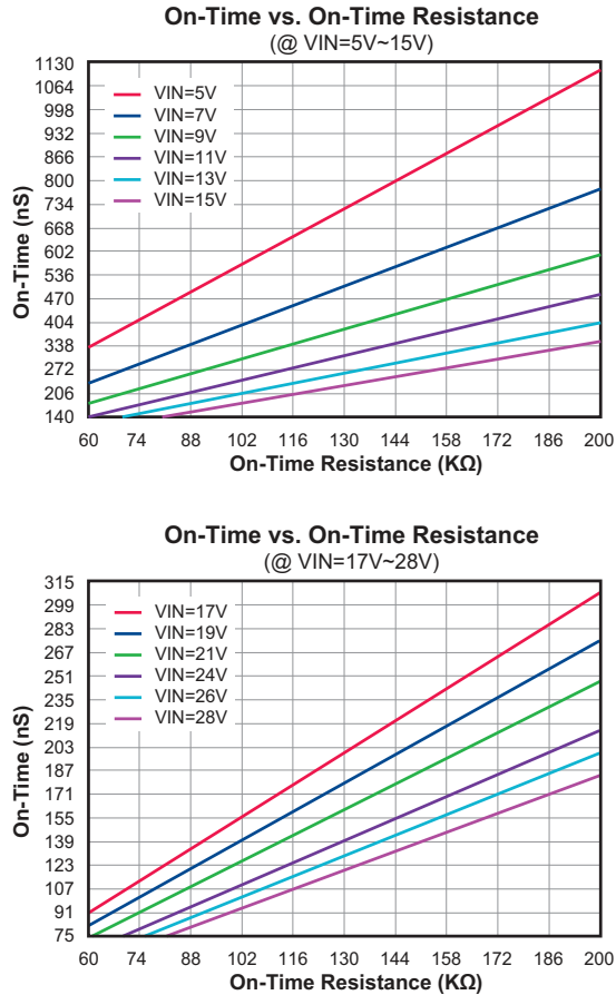
Figure 3. T_{ON} vs. R_{TON} Curves
