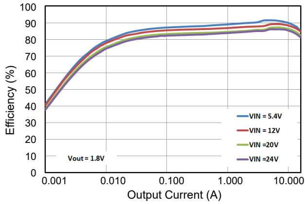
Figure 1. Efficiency vs. Load Current ( V_{OUT} = 1.8V )
