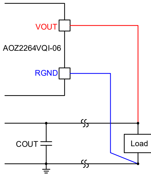
Figure 8. Remote Sensing Connection
