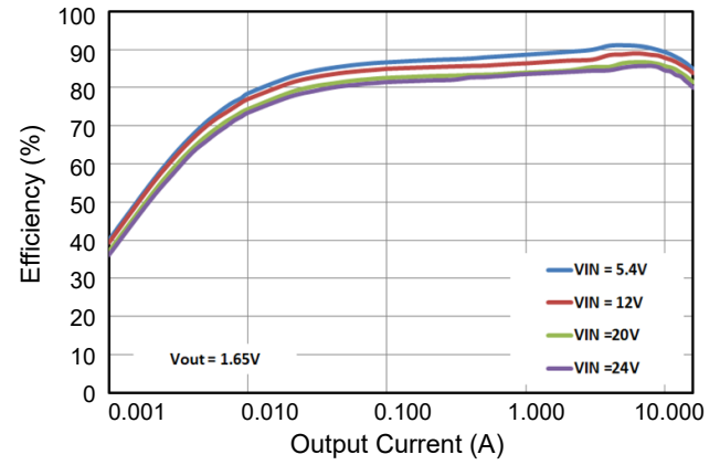
Figure 2. Efficiency vs. Load Current ( V_{OUT} = 1.65V )
