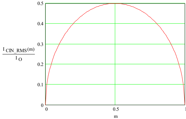
Figure 9. I_{CIN} vs. Voltage Conversion Ratio
