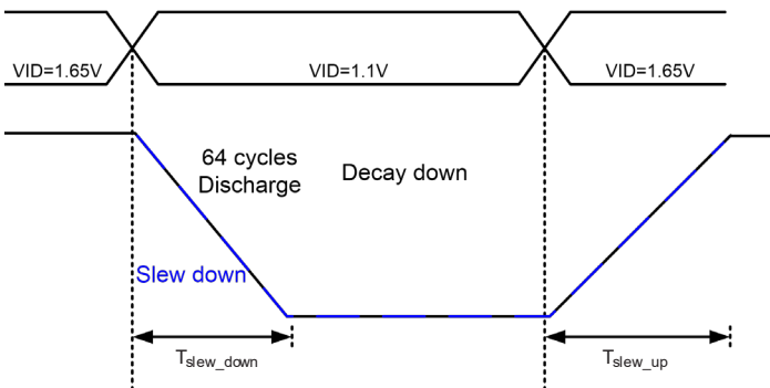
Figure 6. Slew Mode Illustration
