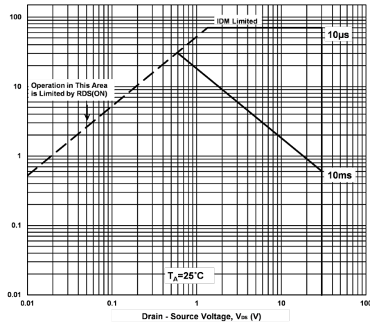
Figure 10. High-Side MOSFET SOA Curve
