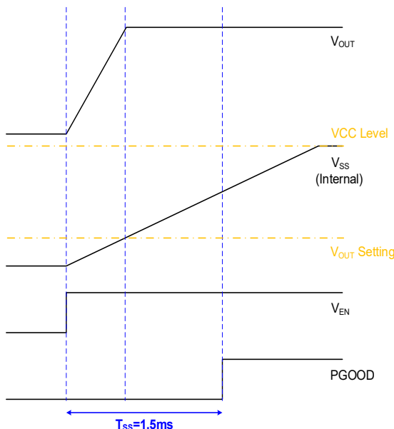
Figure 3. Soft Start Sequence
