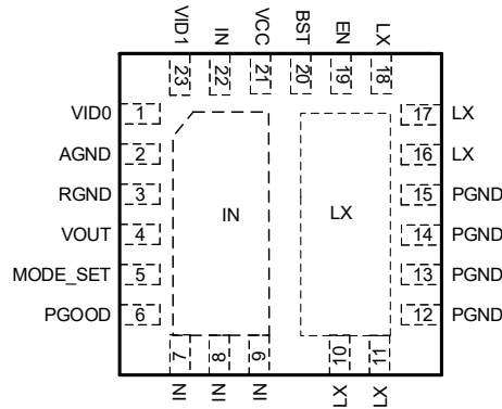
AOZ2264VQI-06 23-pin 4mm x 4mm QFN
