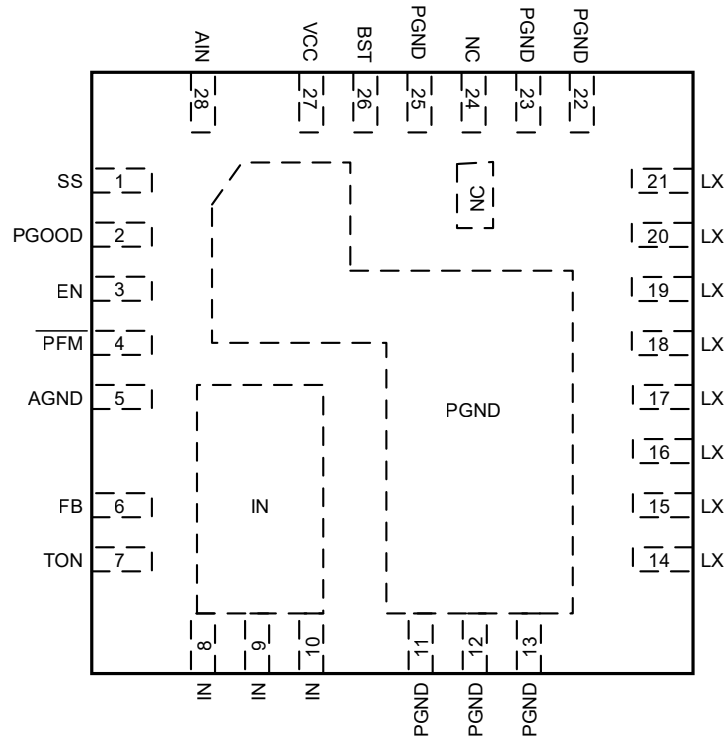
AOZ2378QI 28-pin 5 mm x 5 mm QFN
