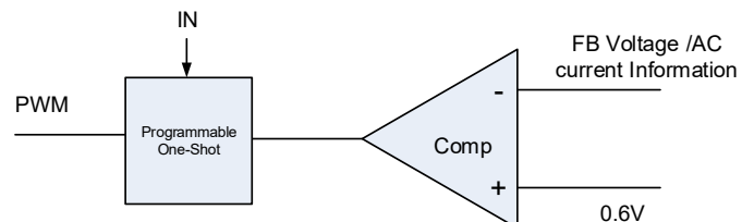
Figure 2. Simplified Control Schematic of AOZ2378QI
