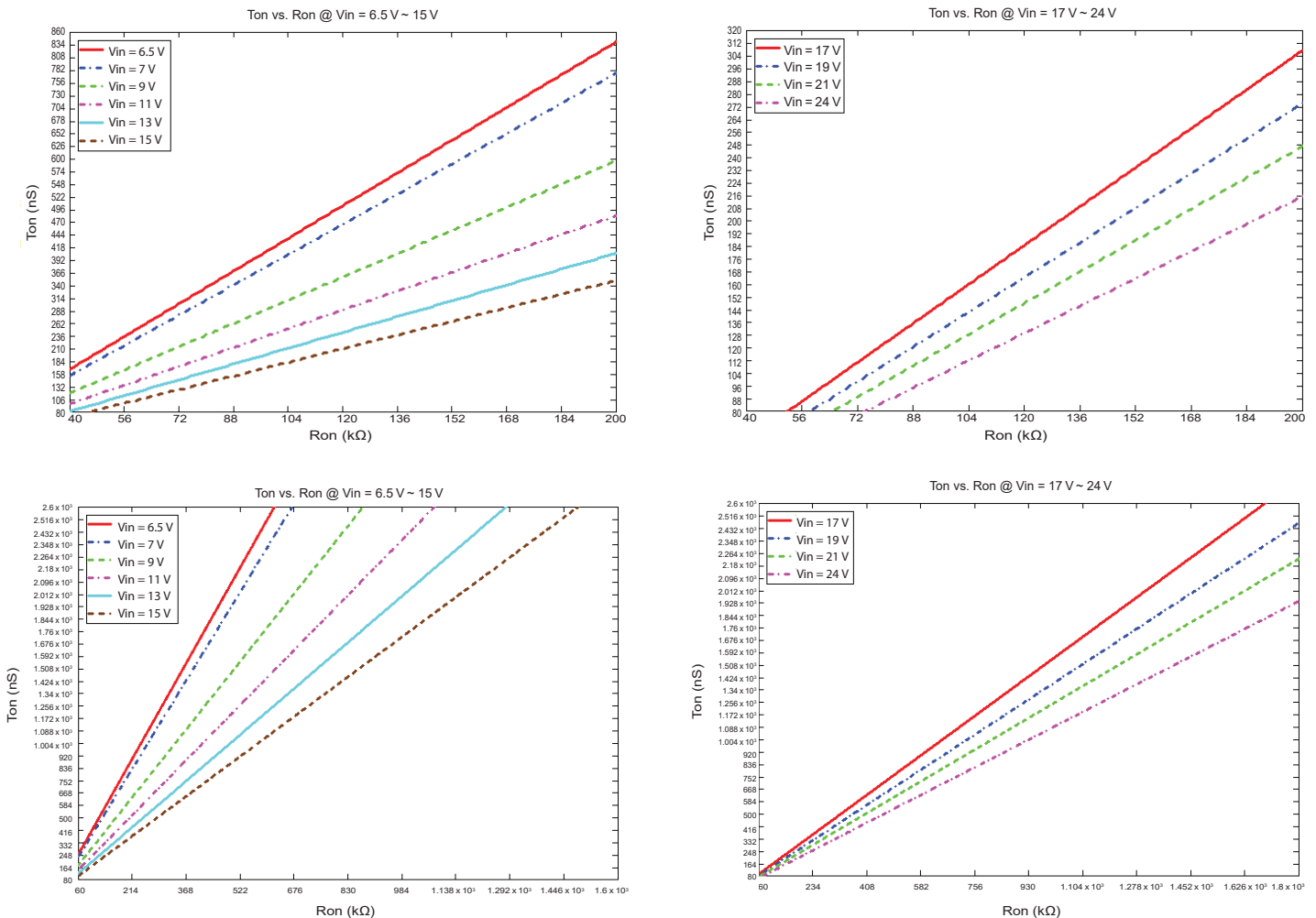
Figure 3. T_{on} vs. R_{on} Curves for AOZ2387QI
