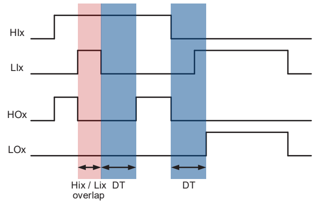
Figure 4. Dead Time and Shoot-Through Prevention
