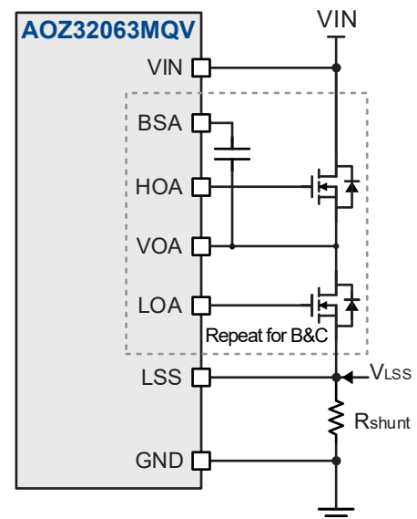
Figure 5. LSS Voltage ( V_{LSS} )
