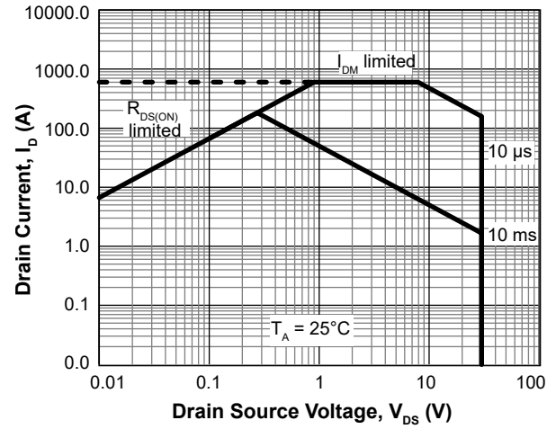
Figure 10. Low-Side MOSFET SOA
