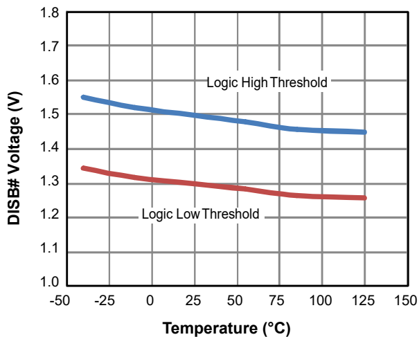
Figure 7. DISB# Threshold vs. Temperature
