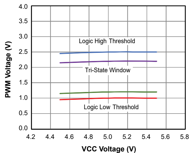
Figure 8. PWM Threshold vs. VCC Voltage
