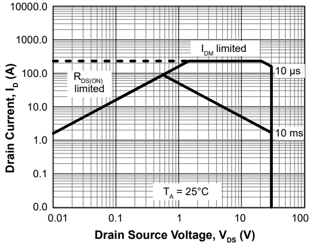
Figure 9. High-Side MOSFET SOA
