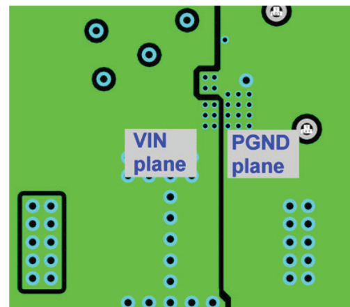
Figure 12. Bottom Layer of PCB
