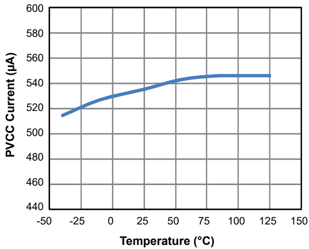
Figure 3. Supply Current ( I_{VCC} ) vs. Temperature
