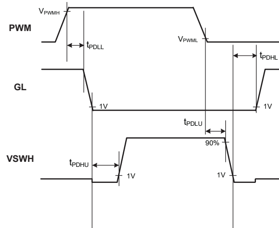
Figure 1. PWM Logic Input Timing Diagram
