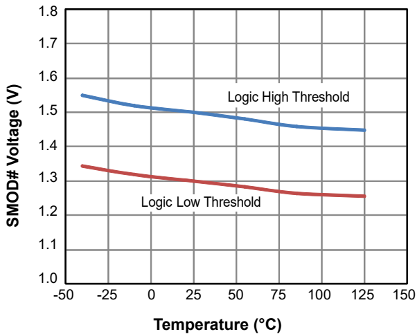
Figure 5. SMOD# Threshold vs. Temperature
