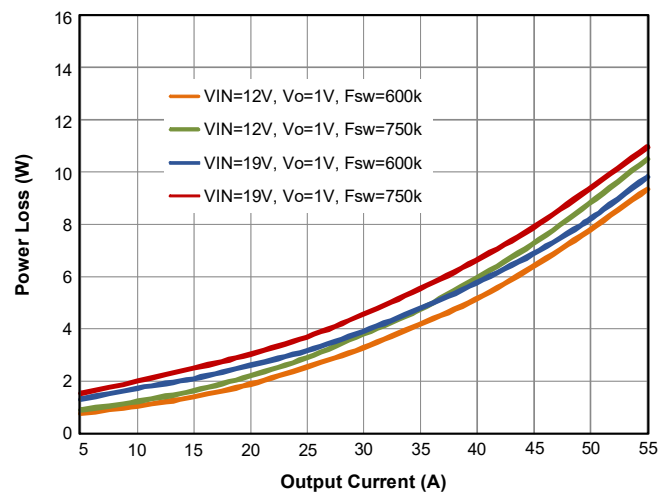
Figure 6. Power Loss vs. Output Current, V_{OUT} = 1.0\text{V}
