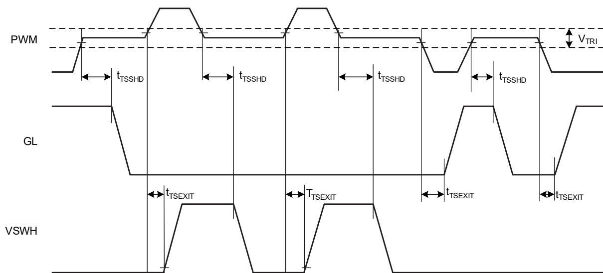
Figure 2. PWM Tri-State Hold Off and Exit Timing Diagramw
