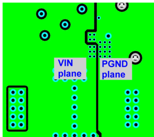
Figure 12. Bottom Layer of PCB
