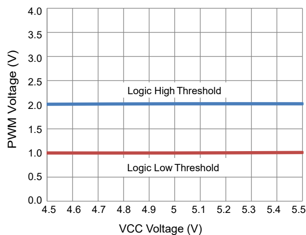
Figure 10. PWM Threshold vs VCC Voltage
