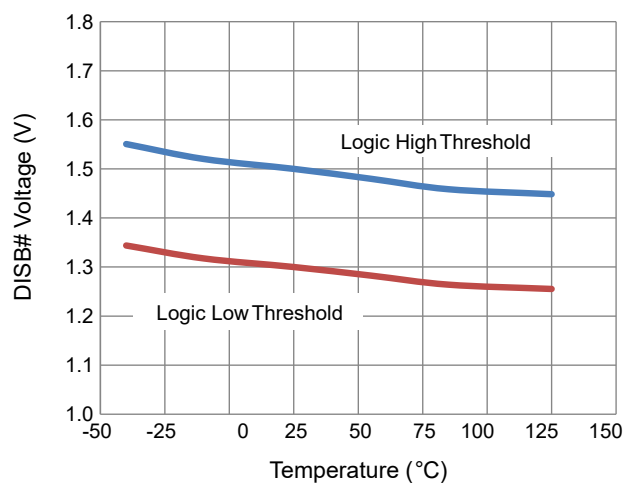
Figure 9. DISB# Threshold vs Temperature
