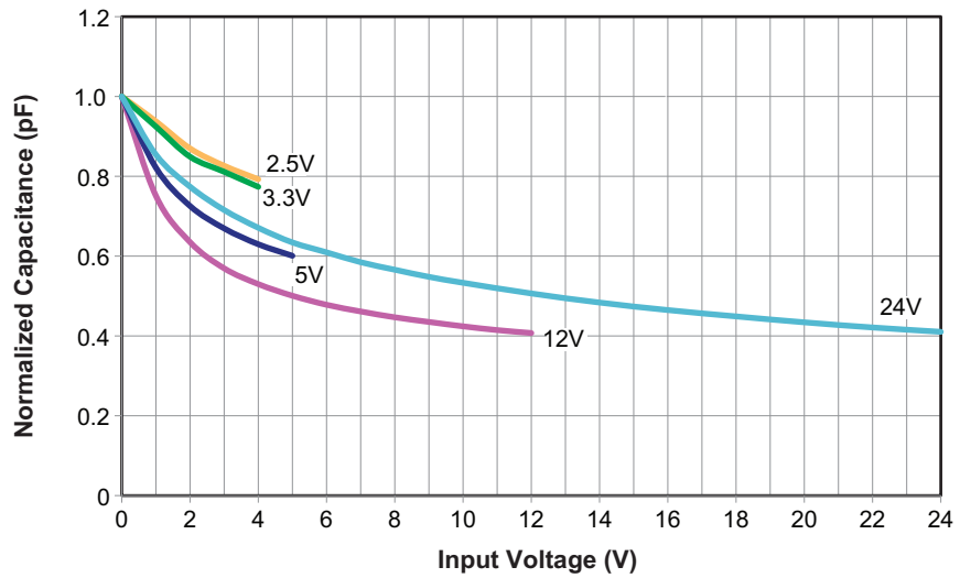
Typical Variation of C_{IN} vs. V_R ( f = 1 \text{ MHz} , T = 25 \text{ }^\circ\text{C} )
