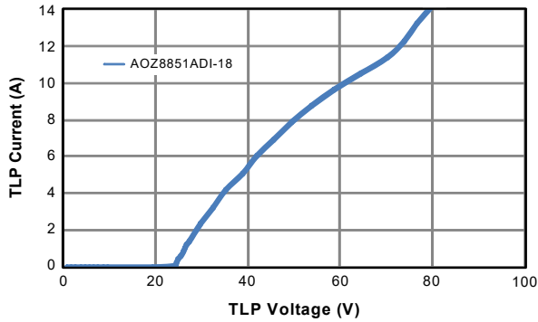
Transmission Line Pulse ( t_p=0.2\text{ns} , t_p=100\text{ns} )
