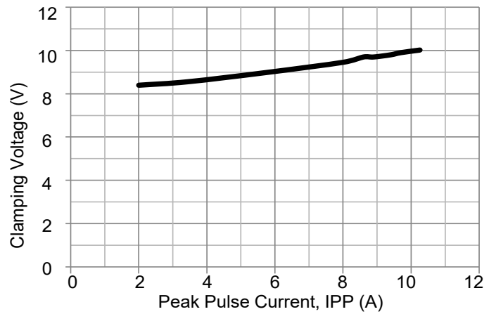
IEC61000-4-5 Surge 8/20 \mu s (Any I/O Pin to Pin)
