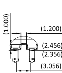
Detail A
