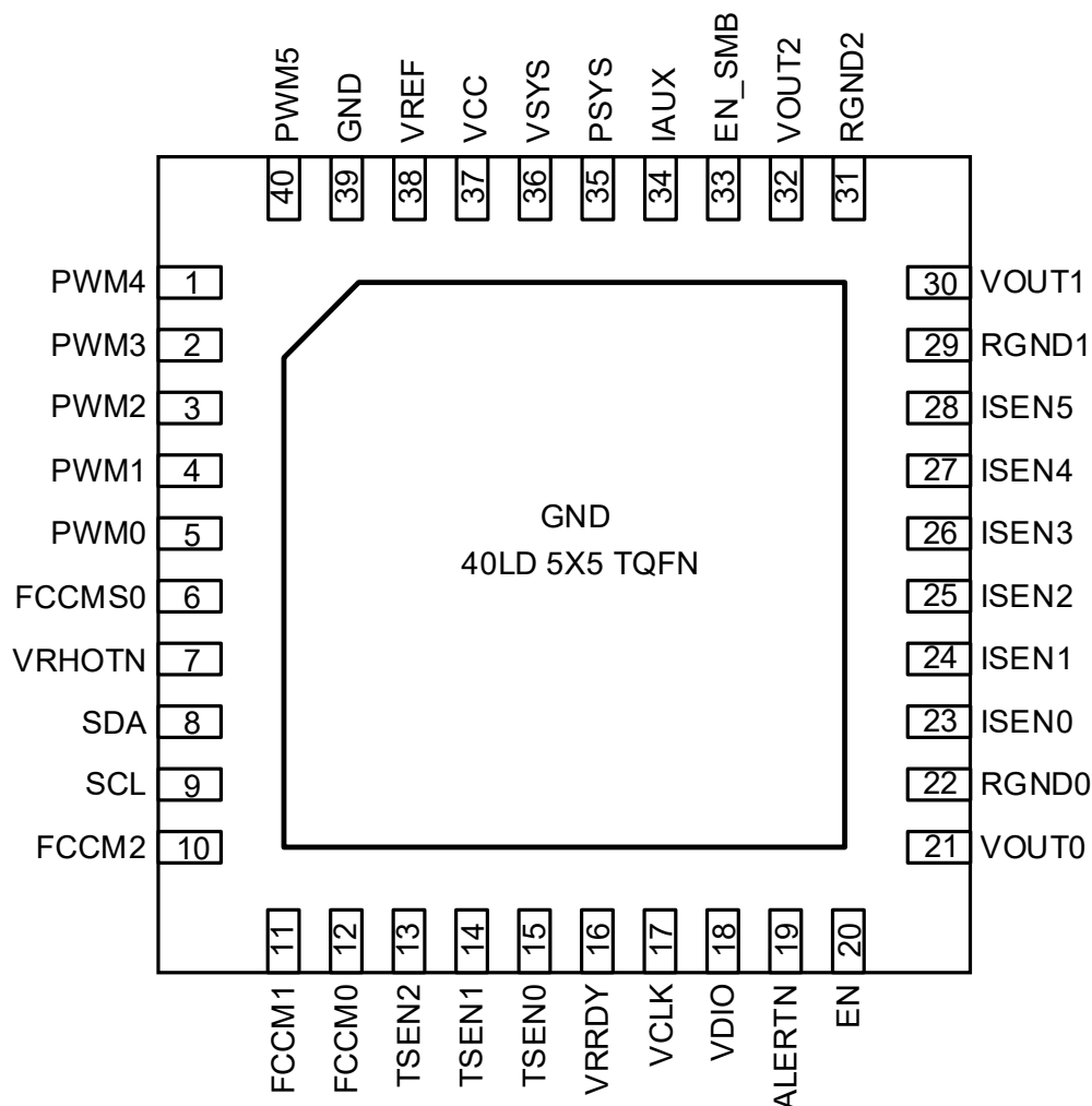
Figure 1. QFN 5x5-40L (Top View)
