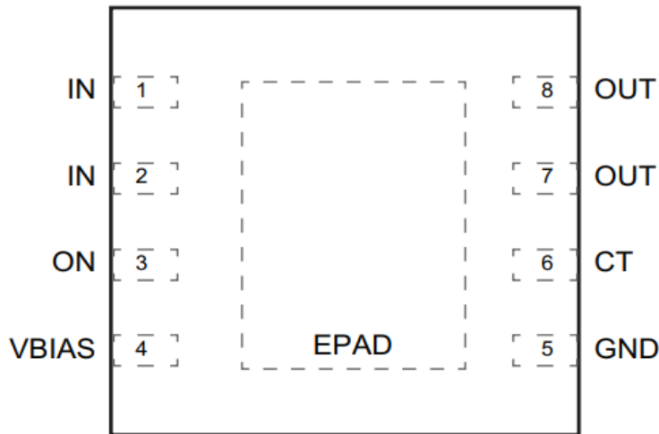
2mm x 2mm DFN-8 (Top View)
