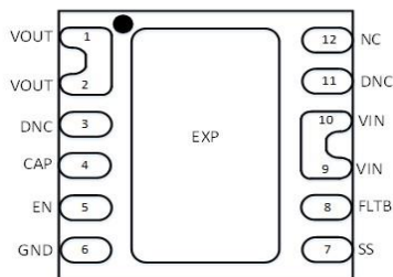
3mm x 3mm DFN-12L (Top Transparent View)
