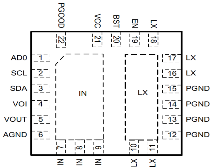
22-Pin 4mm x 4mm QFN
