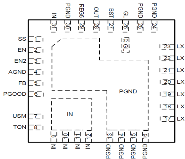
31-Pin 4mm x 4mm QFN
